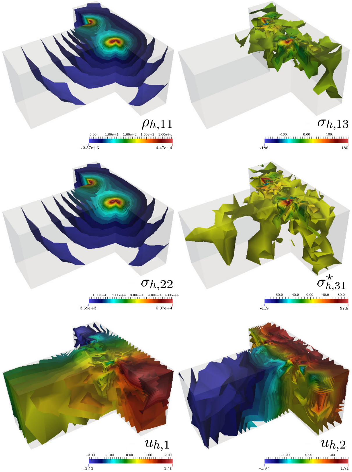
Figure 5.6: Example 3, iso-surfaces of some components of the approximate solutions ( k = 2 and N = 270037 ) for adaptive scheme.
