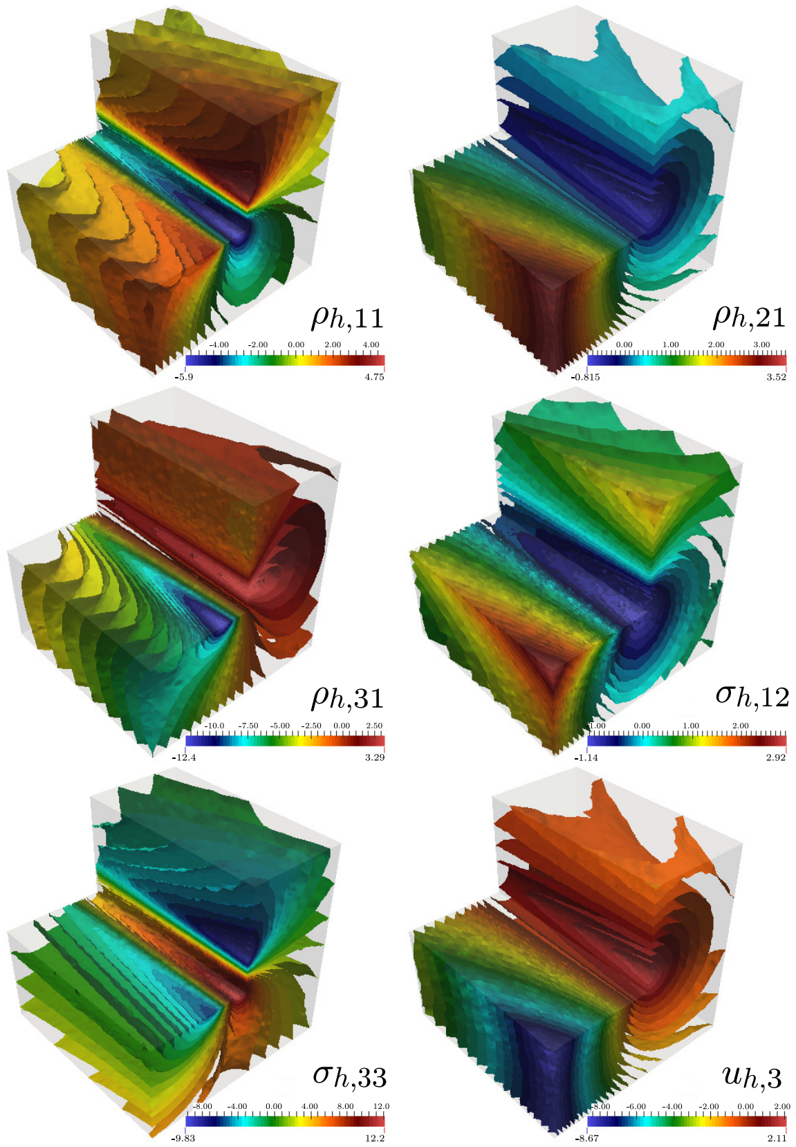
Figure 5.3: Example 2, iso-surfaces of some components of the approximate solutions ( k = 0 and N = 2251543 ) for adaptive scheme.
