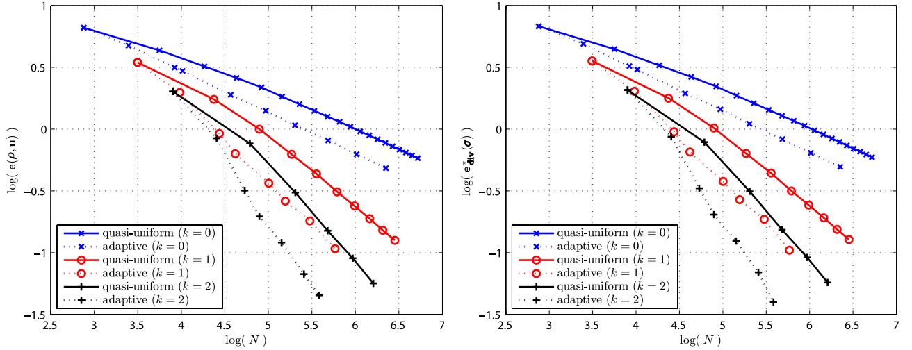
Figure 5.1: Example 2, e(\rho, u) vs. N (left) and e_{\text{div}}^*(\sigma) vs. N (right).
