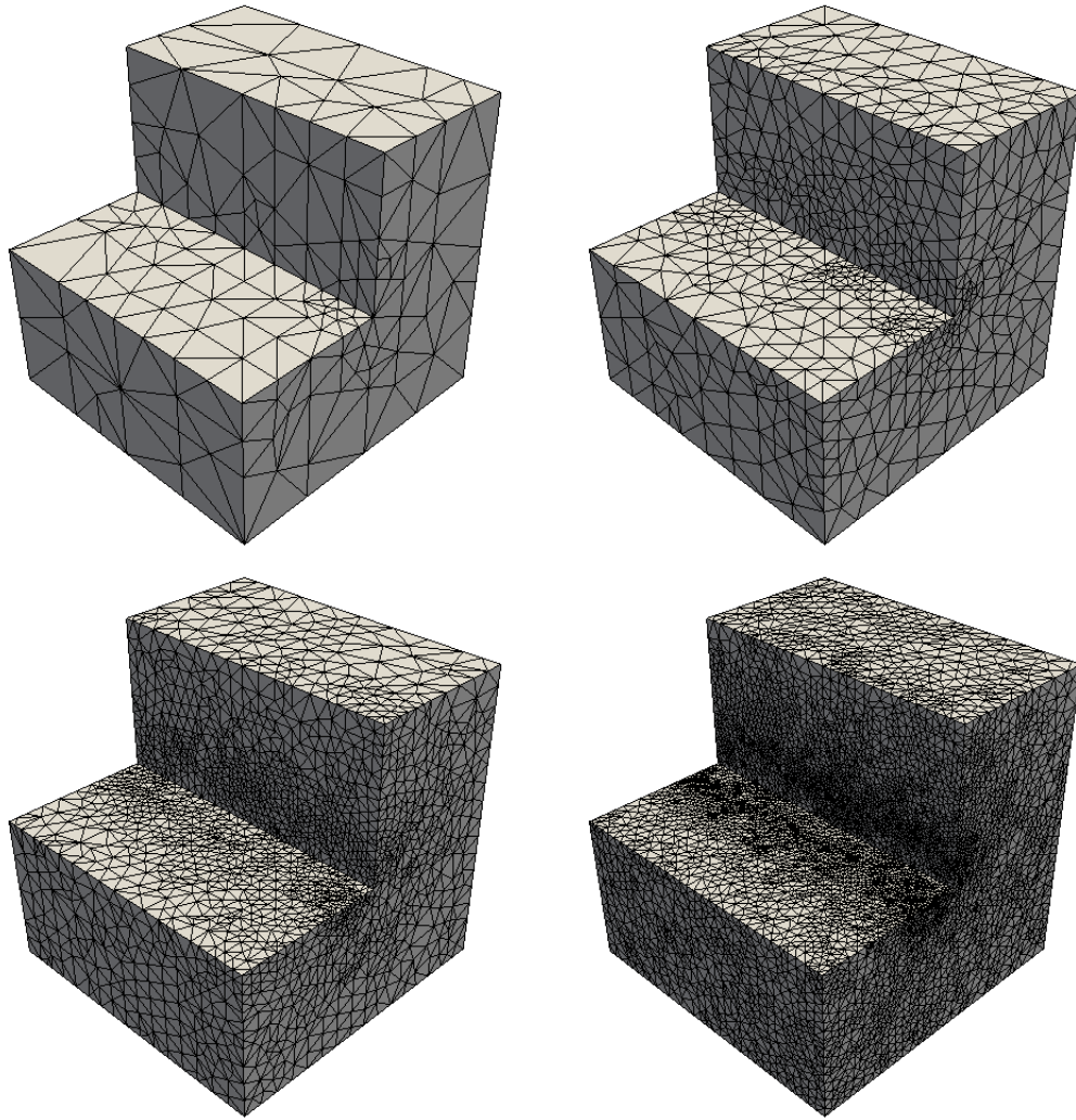
Figure 5.2: Example 2, adapted meshes for k = 0 with 10348, 93637, 485527, and 2251543 degrees of freedom.
