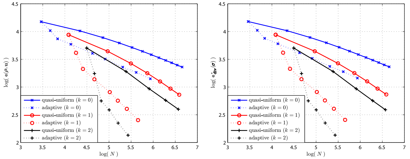
Figure 5.4: Example 3, e(\rho, \mathbf{u}) vs. N (left) and e_{\text{div}}^*(\sigma) vs. N (right).
