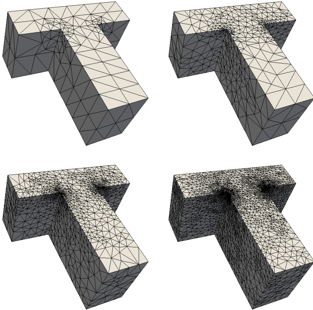
Figure 5.5: Example 3, adapted meshes for k = 0 with 6868, 42169, 204958, and 861778 degrees of freedom.
